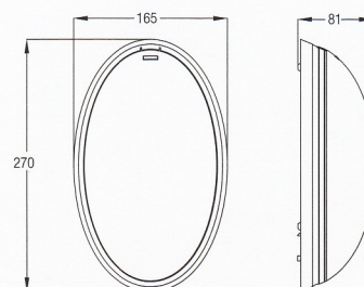
400-014-107 Ninova Wall Fixture (Maple)
